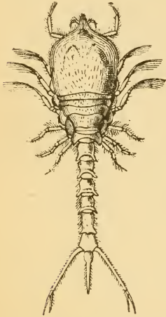
FIG. 26.— Diastylis Goodsi , dorsal view of female [Hansen].
