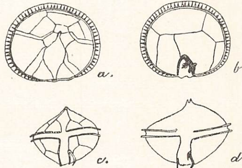
Fig. 12. Peridinium decipiens 833 3 .
