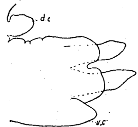
FIG. 49.—Parapodium of Glycera abbranchiata . d. c. and v. c., dorsal and ventral cirri.
