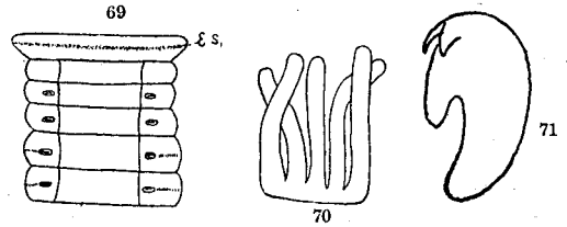
FIGS. 69-71.— Thelepus crassibranchiatus . Fig. 69, Anterior portion, \times 20 : e. s., eye spots. Fig. 70, Branchia of second segment, \times 13 . Fig. 71, Uncinate seta, \times 428 .
