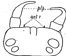
FIG. 4.—Head of Castalia mutilata , \times 26 ; ant? , antennæ; plp. , palps.
