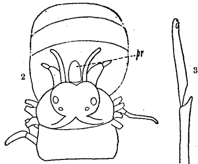
FIGS. 2, 3.— Castalia longicirrata . Fig. 2, Head, \times 14 ; pr. , process on proboscis. Fig. 3, Compound seta, \times 95 .
