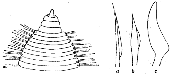
FIG. 67.—Anterior end of Cirratulus elongatus , \times 23 .
