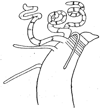
FIG. 66.—Anterior portion of Cirratulus nigromaculata , \times 5 .
