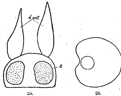
FIGS. 25, 26.— Phyllodoce magna-oculata . Fig. 25, Head, \times 70 ; d. ant. , dorsal antennæ; e , eye. Fig. 26, Gill, \times 70 .
