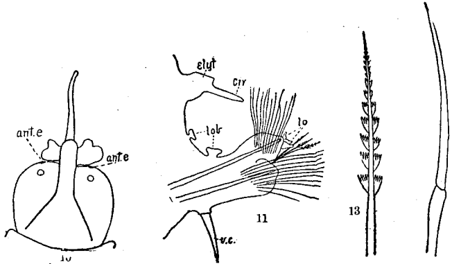
FIGS. 10-13.— Sthenelais grubel . Fig. 10, Head, \times 21 ; ant. e. , anterior eyes. Fig. 11, Parapodium, \times 18 ; v. c. , ventral cirrus; cir. , dorsal cirrus; elyt. , elythrophere; lob. , processes on parapodium. Fig. 12, Compound ventral seta, \times 143 . Fig. 13, Complex ventral seta, \times 143 .
