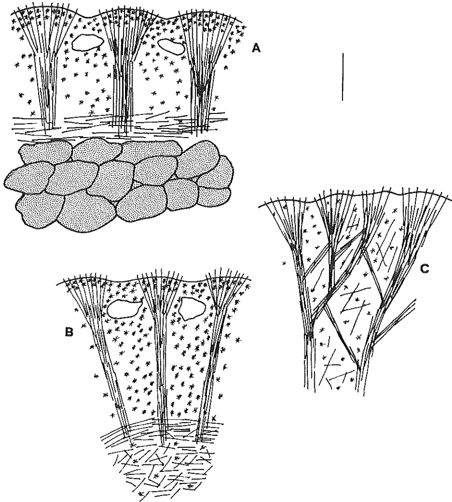
Figure 2. Skeletal arrangement in the genera: A, Columnnitis ; B, Nucleotethya ; C, Tectitethya . Bar: 1 mm.
