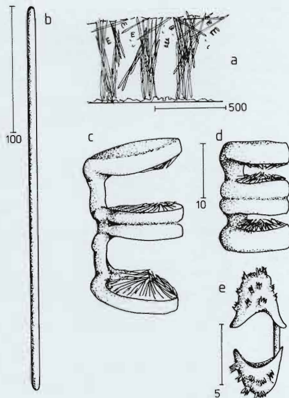
Figure 1: Tetrapocillon atlanticus n.sp., a cross section of choanosome; b. strongyle, c. larger tetrapocilla, d. smaller tetrapocilla, e. spined isochela (all scale in \mu\text{m} ).
